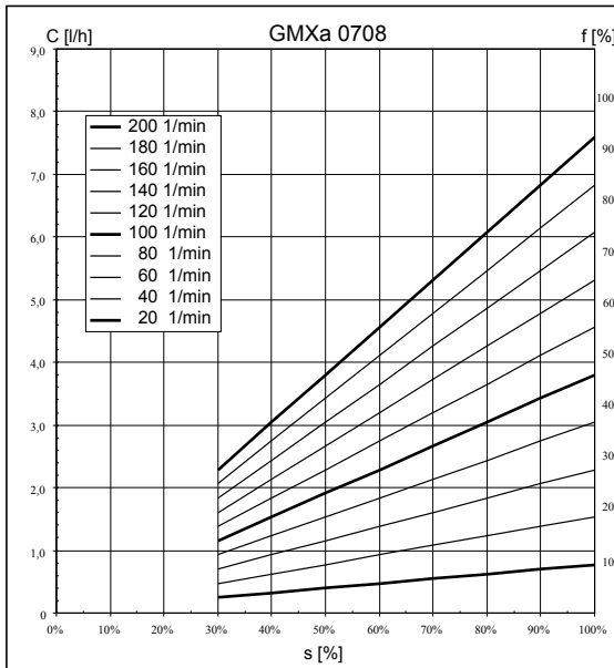
Fig. 1: Capacity C at medium back pressure depending on the stroke length s for different stroke rates f
